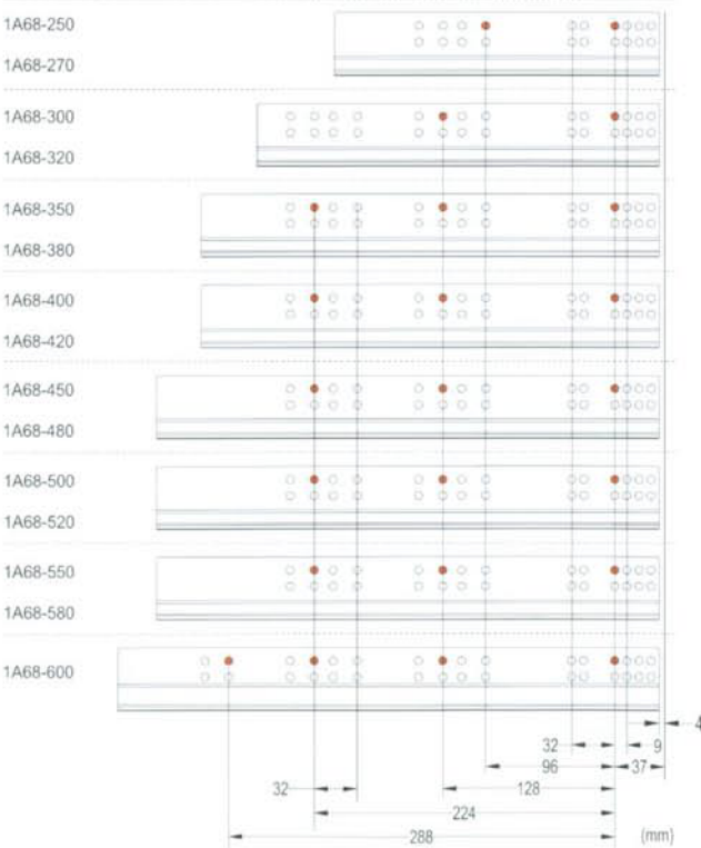
Cabinet Holes Position
